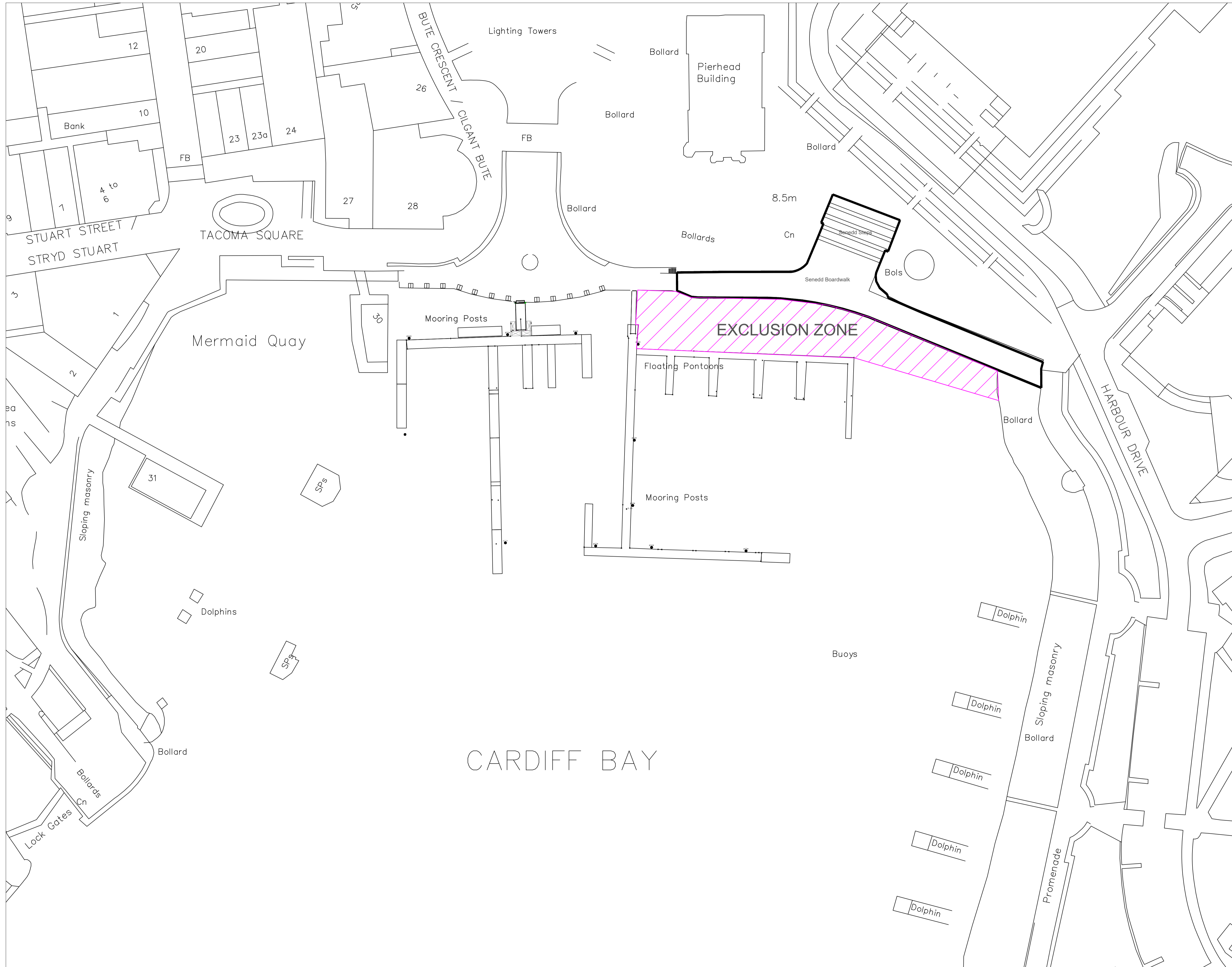
LAYOUT PLAN
